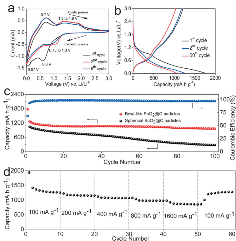
Figure 3. Electrochemical measurements of the bowl-like \text{SnO}_2 @C nanocomposite: a) representative cyclic voltammograms (CVs) at a scan rate of 0.5 \text{mV s}^{-1} ; b) charge-discharge voltage profiles for the 1 st , 2 nd , and 50 th cycles at a current density of 400 \text{mA g}^{-1} ; c) cycling performance at a current density of 400 \text{mA g}^{-1} and the coulombic efficiency; d) rate performance.
